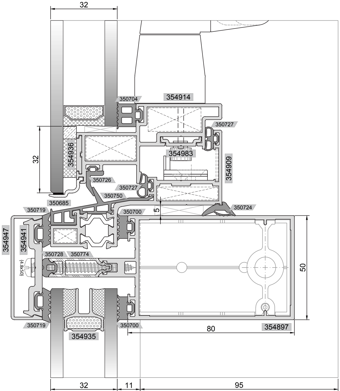
YATAY DETAYI HORIZONTAL DETAIL
