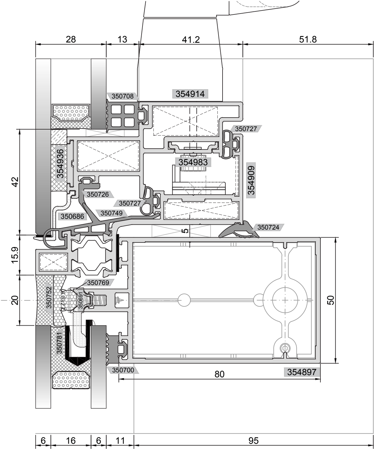
YATAY DETAYI HORIZONTAL DETAIL
