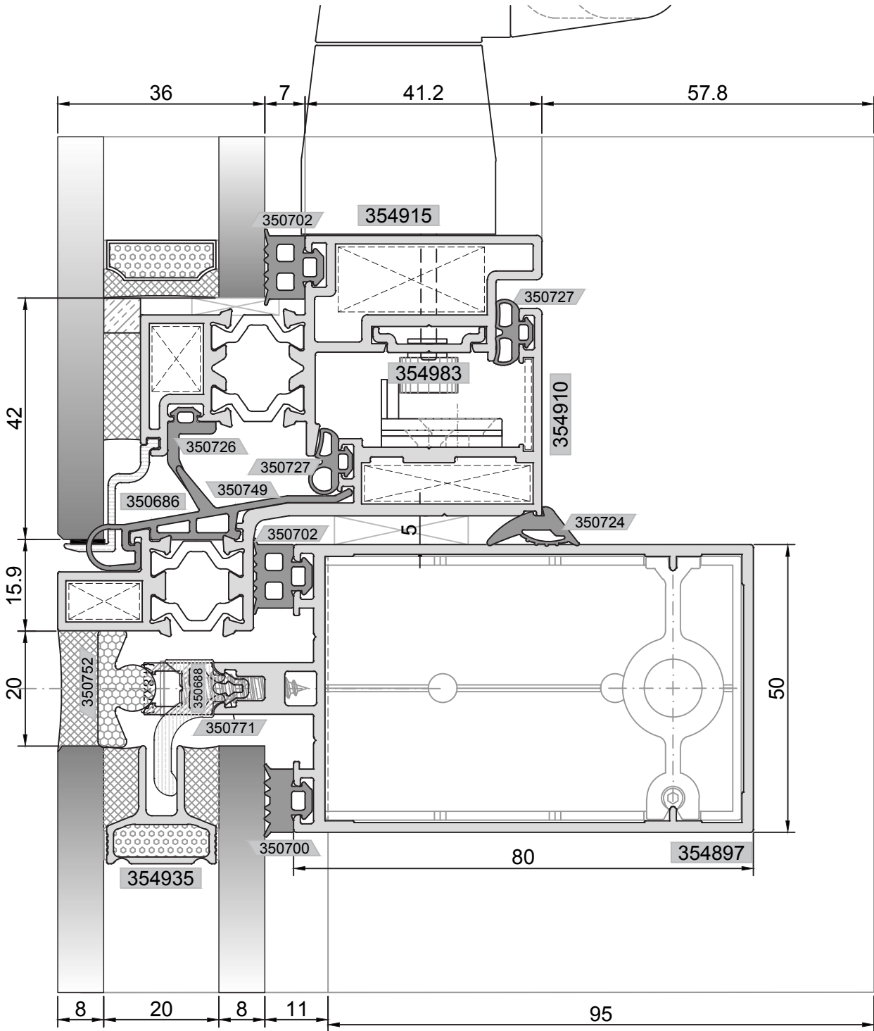
ALTERNATİF 2: YALITIMLI KANAT DETAYI ALTERNATIVE 2 : INSULATED VENT DETAIL
