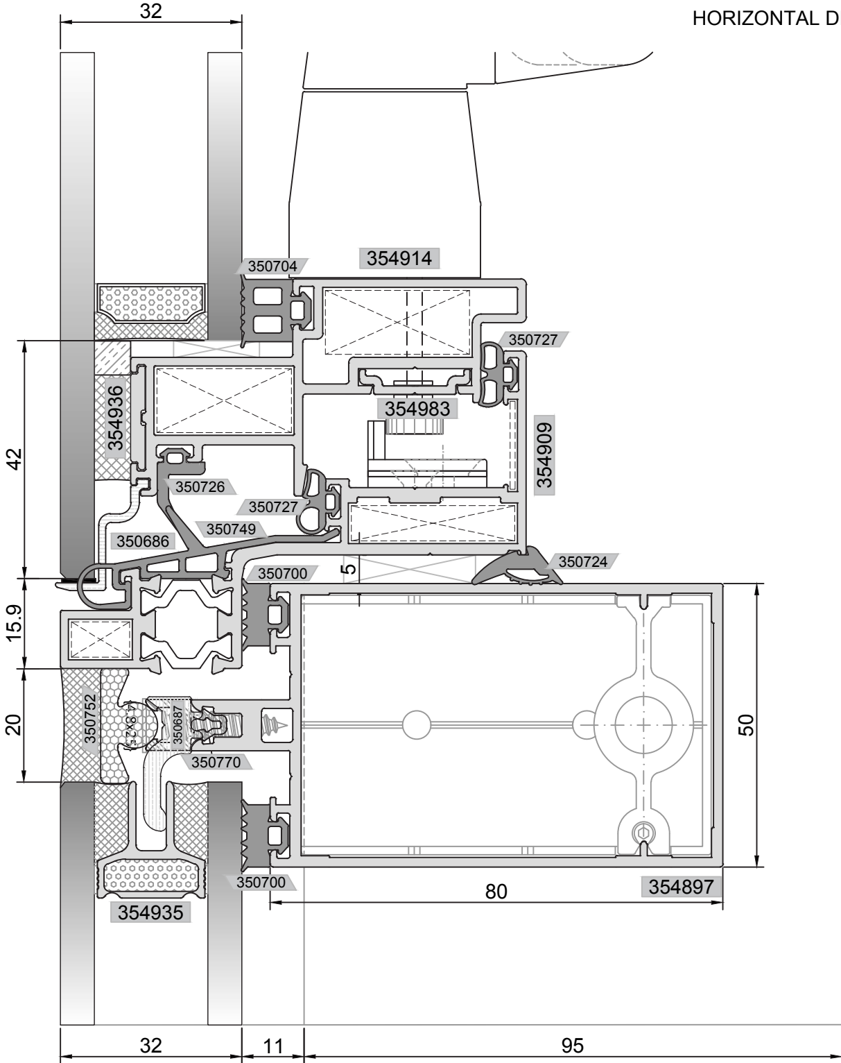
ALTERNATİF 1: YALITIMSIZ KANAT DETAYI ALTERNATIVE 1 : UNINSULATED VENT DETAIL
