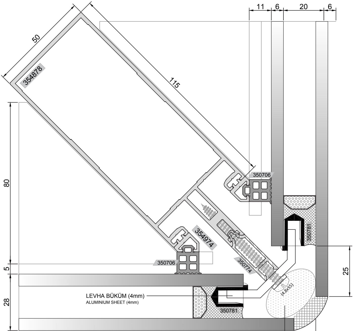
ALTERNATİF 1: TEK DİKMELİ KÖŞE DETAYI ALTERNATIVE 1 : CORNER DETAIL WITH SINGLE MULLION
