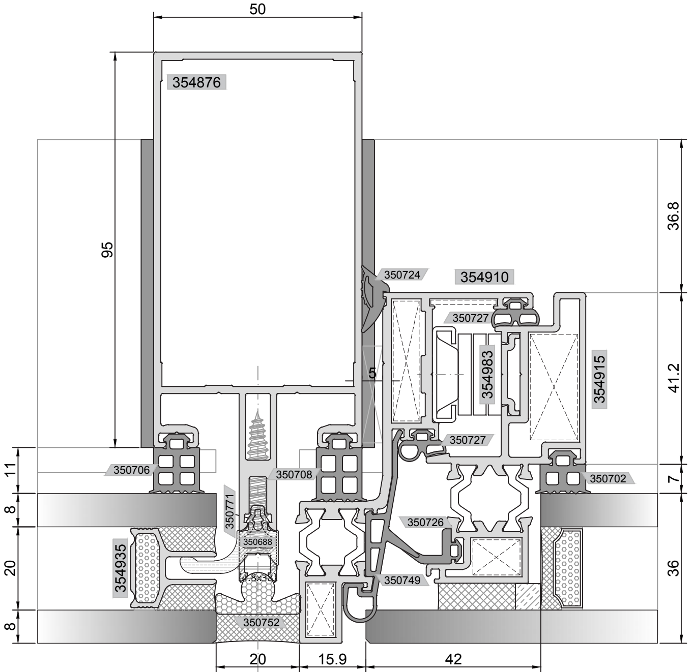
ALTERNATİF 2: YALITIMLI KANAT DETAYI ALTERNATIVE 2 : INSULATED VENT DETAIL
