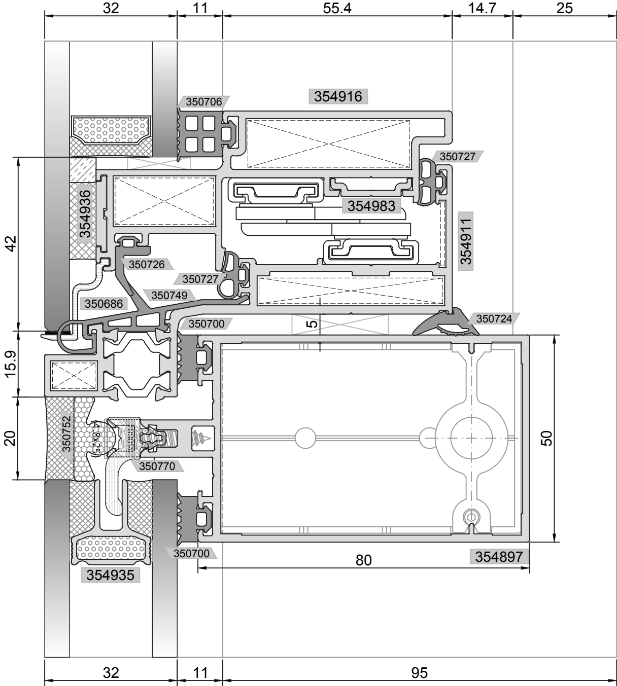
ALTERNATİF 2: YALITIMSIZ PARALEL AÇILIR KANAT DETAYI ALTERNATIVE 2 : PARALEL OPENING UNINSULATED VENT DETAIL
