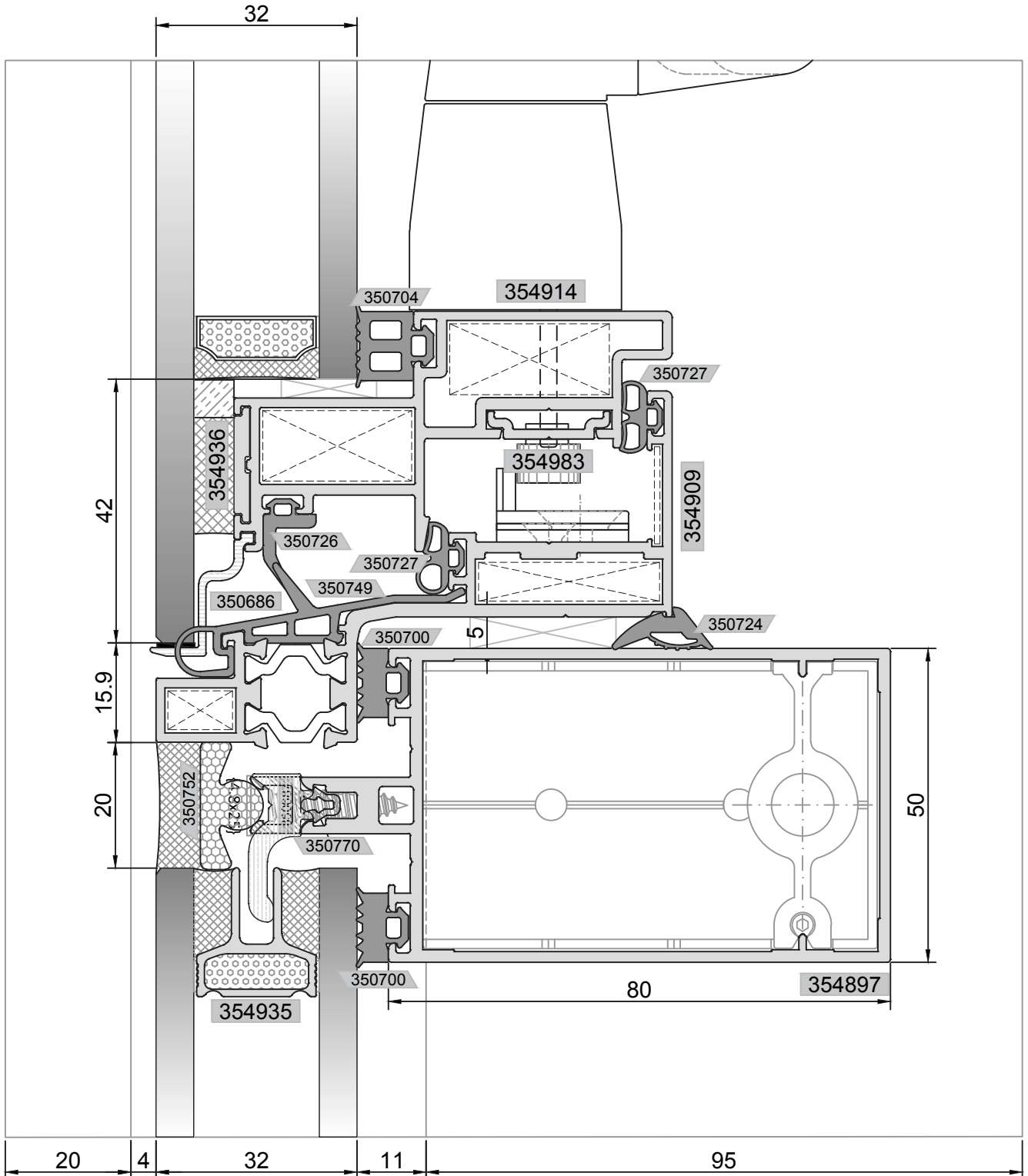
YATAY DETAYI HORIZONTAL DETAIL
