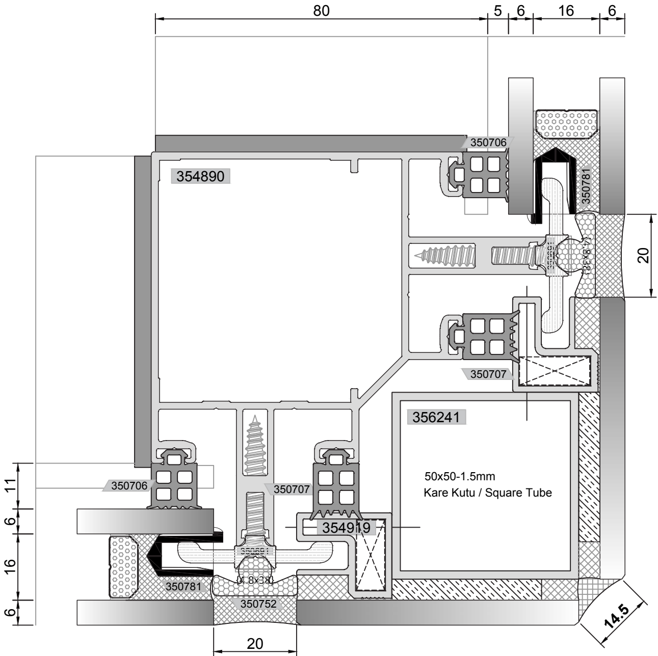
ALTERNATİF 2: ÇİFT DİKMELİ KÖŞE DETAYI ALTERNATIVE 2 : CORNER DETAIL WITH DOUBLE MULLION
